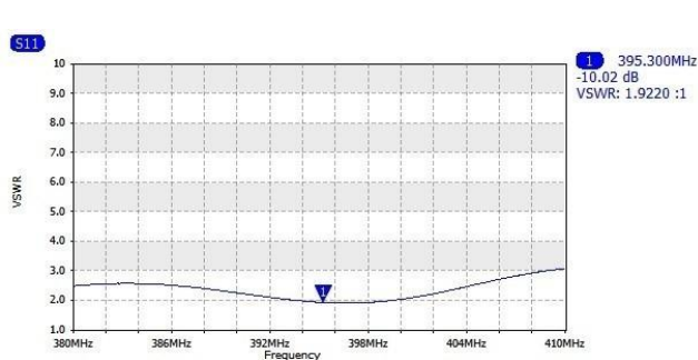
Typical SWR w/o matching box
