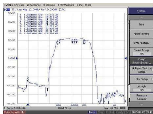
Gain GPS/GLONASS/GALILEO
